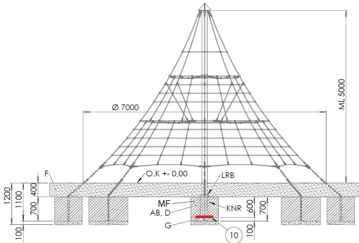
Side view with foundations
